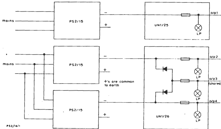
Fig. 1 Block Diagram of the PS2/16
