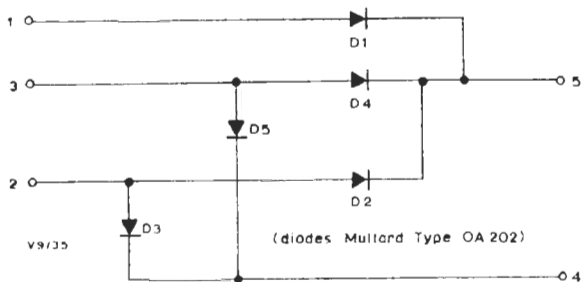
Fig. 25.1 Diode Network NE1/508
