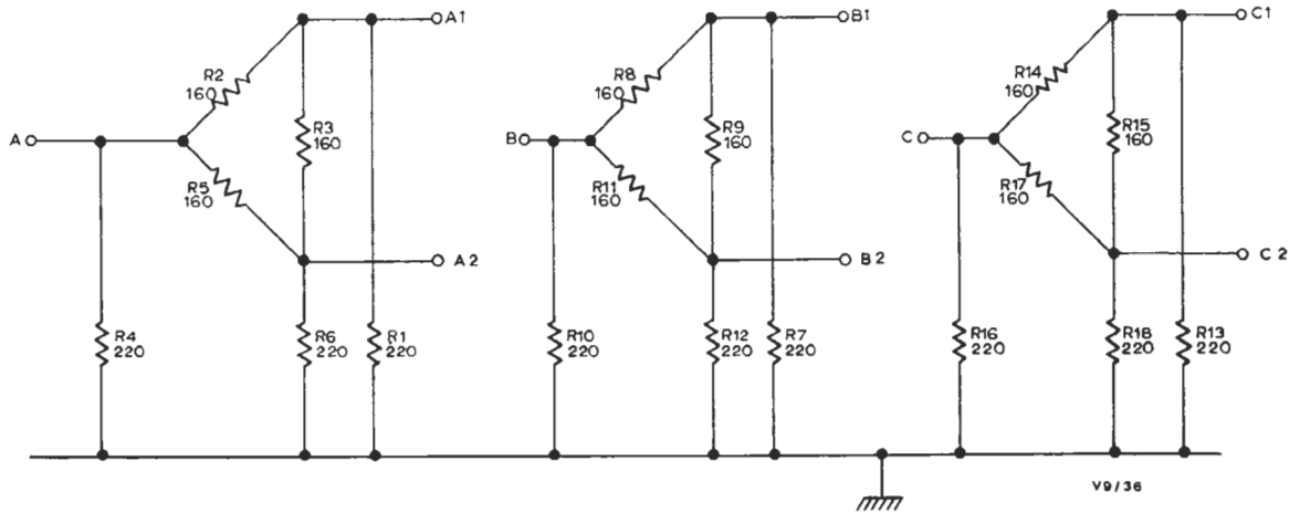
Fig. 26.1 Circuit of the AT3/504
