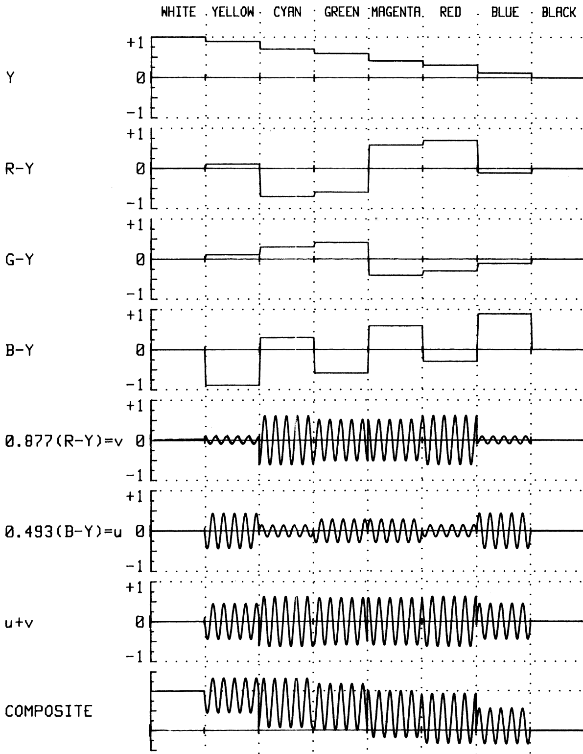
THEORETICAL WAVEFORMS FOR A SET OF COLOUR BARS
